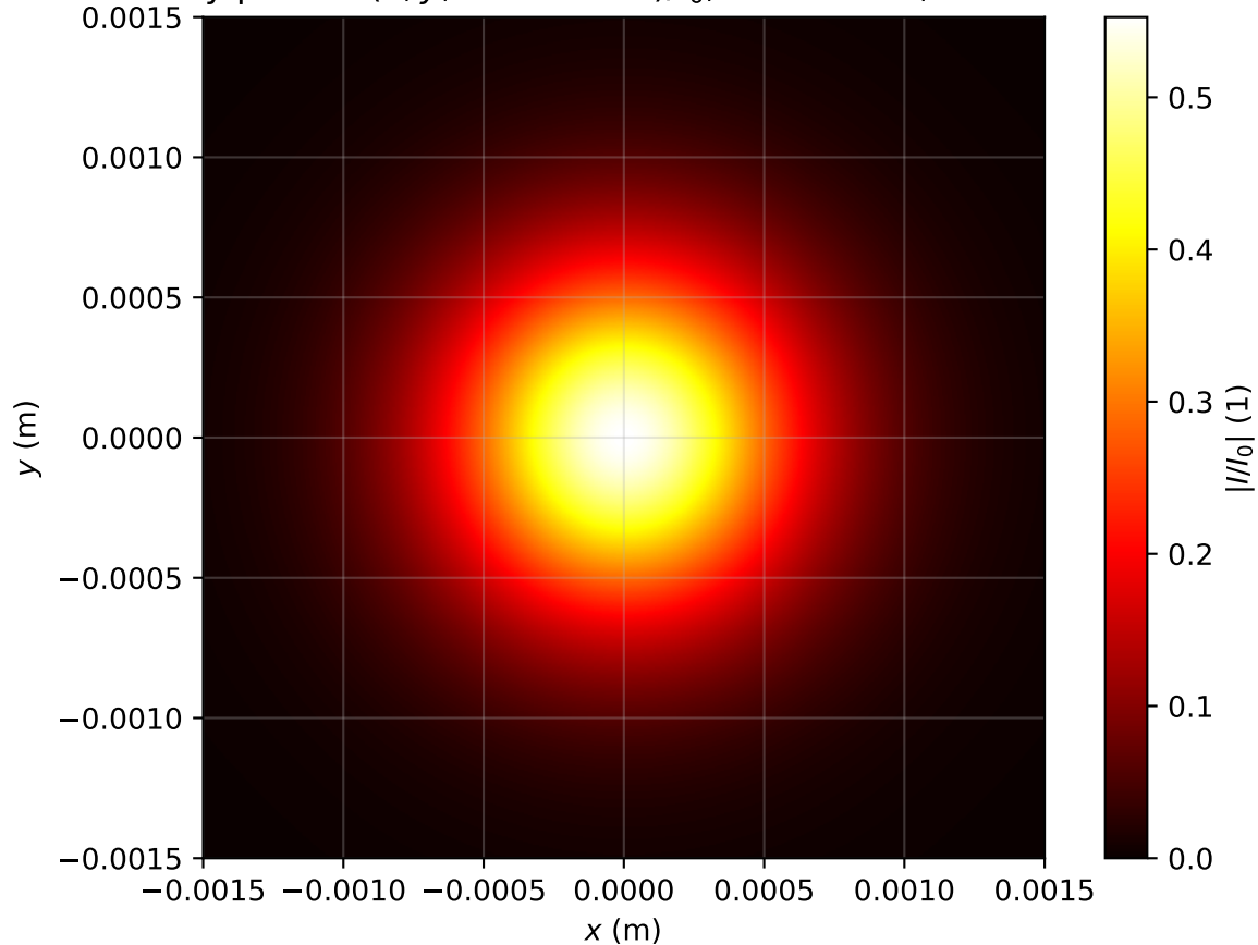
Intensity profile I(x, y, z = 3.582m)/I_0 , \text{Pin}=0.6\text{Pcr} , artificial time
